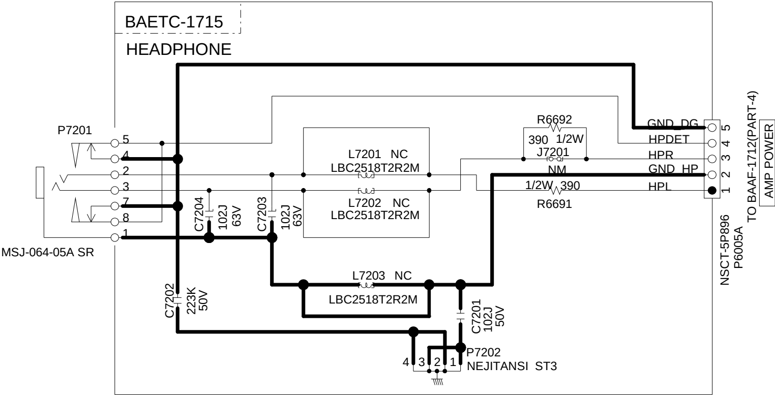
MODEL NO.TX-SR343/444 , HT-R494 SCHEMATIC DIAGRAM (PART-8) HEADPHONE SECTIC
