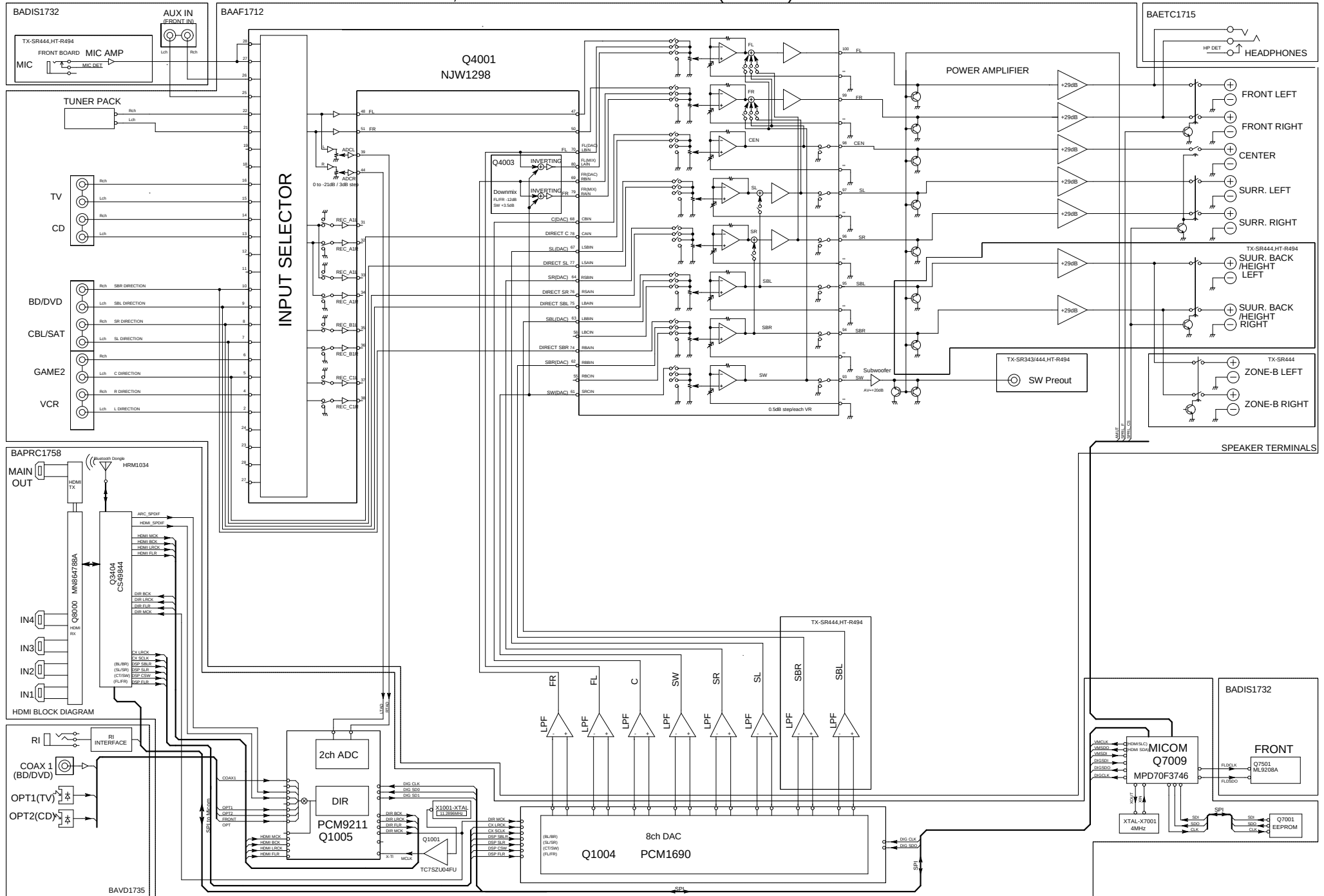
MODEL NO. TX-SR343/444,HT-R494 BLOCK DIAGRAM (PART-1) AUDIO SECTION
