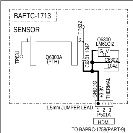
MODEL NO. TX-SR343/444,HT-R494 SCHEMATIC DIAGRAM AMP SECTION (PART-4)
