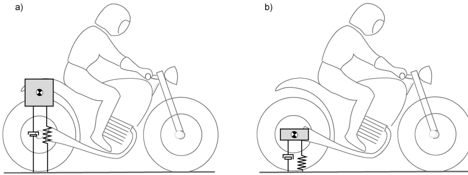
Figure 1.16 Half-vehicle model with 1DOF for sprung mass a), and for unsprung mass b).
