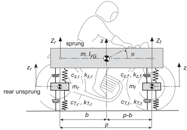
Figure 1.18 Full-vehicle model with four DOF.
