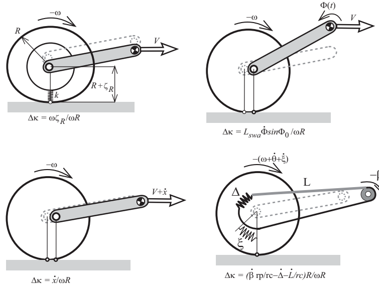
Figure 1.22 Mechanisms generating longitudinal fluctuating slips.
