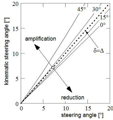
Figure 1.3 Kinematic steering angle \Delta as a function of the handlebar steering angle \delta .
