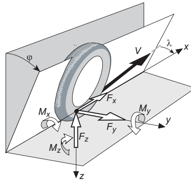
Figure 1.4 Tyre forces and torques.
