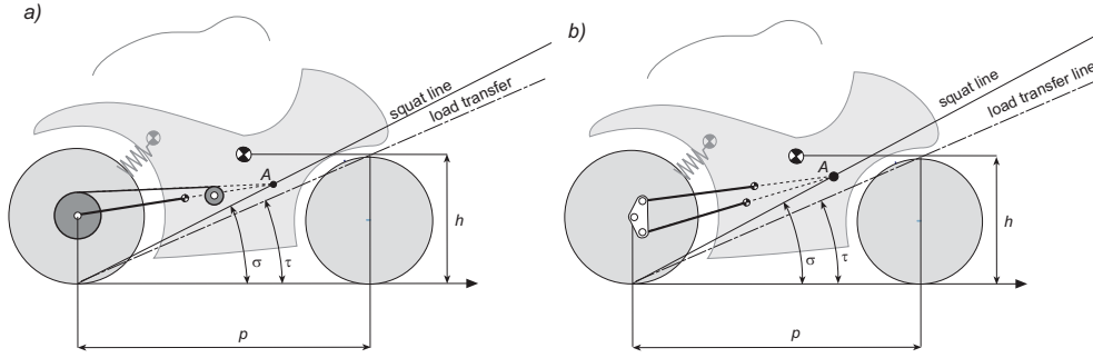
Figure 1.20 Squat and load transfer lines.
