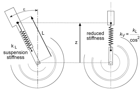
Figure 1.13 Reduced stiffness for the telescopic fork.
