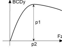
Figure 1.7 Tyre cornering stiffness as a function of normal load.
