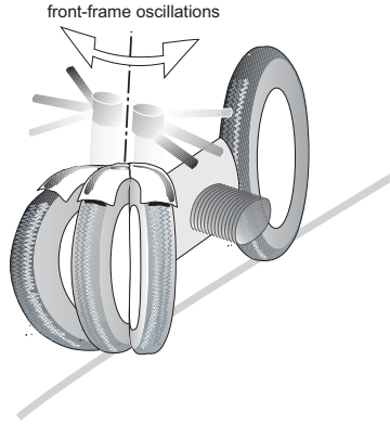
Figure 1.27 Wobble mode.
