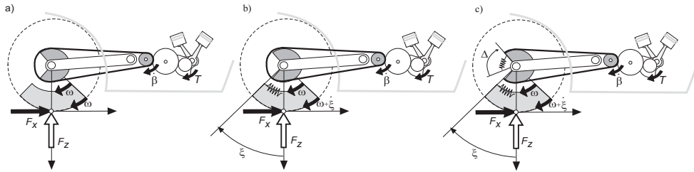
Figure 1.21 Half-vehicle model.
