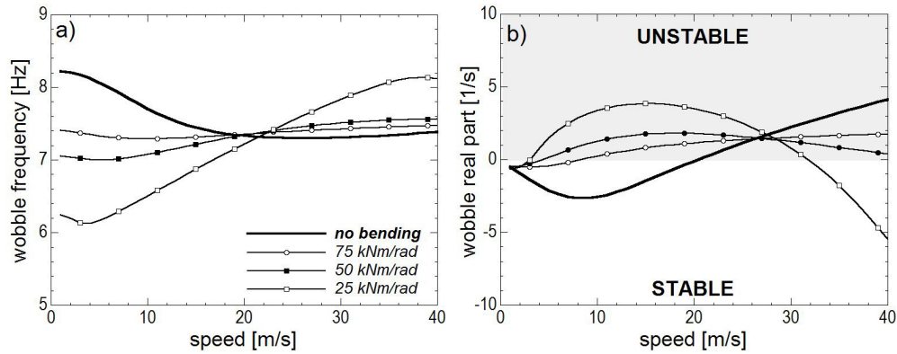
Figure 1.29 Effect of front bending on wobble.
