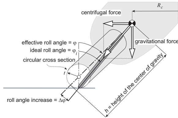
Figure 1.23 Roll equilibrium.
