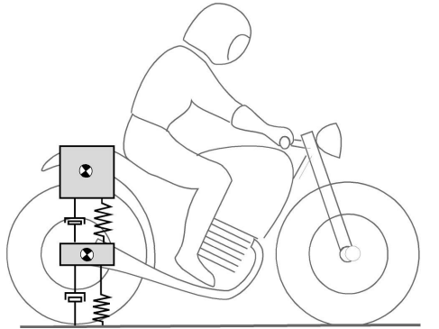
Figure 1.17 Half-vehicle model with 2DOF.
