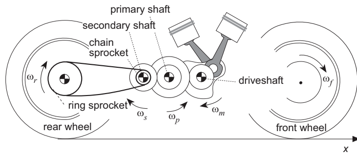
Figure 1.19 Motorcycle powertrain.
