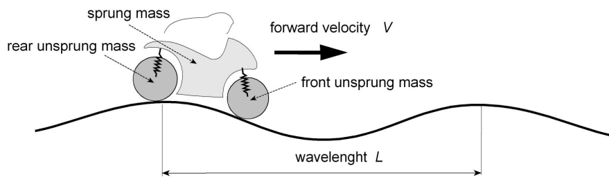
Figure 1.14 Road undulation.
