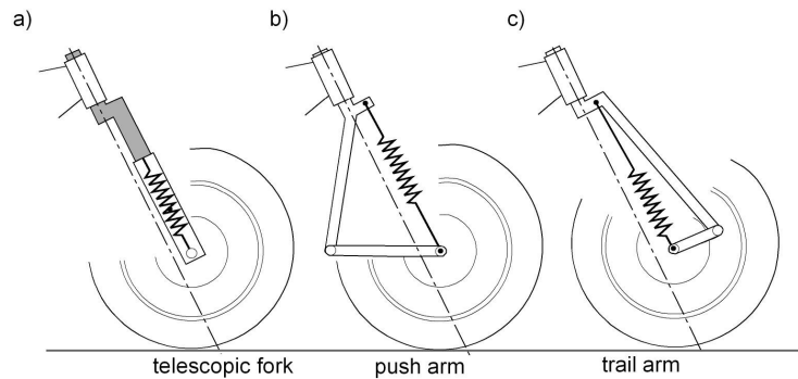
Figure 1.11 Example of front suspensions.
