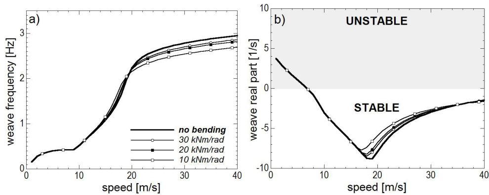
Figure 1.30 Effect of rear bending on weave.
