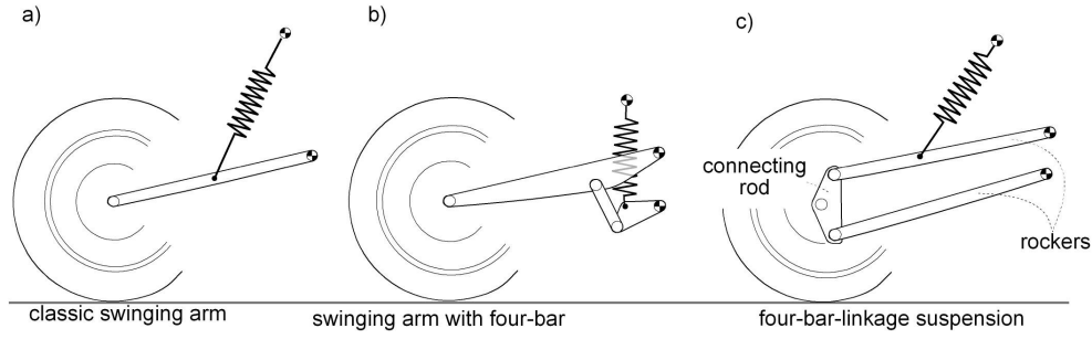
Figure 1.12 Example of rear suspensions.
