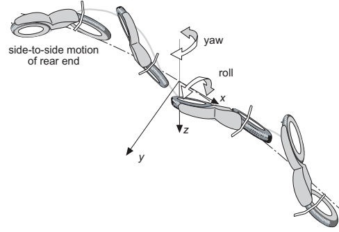
Figure 1.26 Weave mode.
