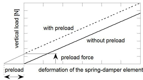
Figure 1.10 Elastic force as a function of preload.
