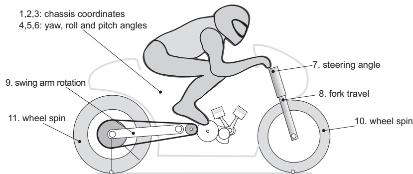
Figure 1.1 Degrees of freedom of a two-wheeled vehicle.
