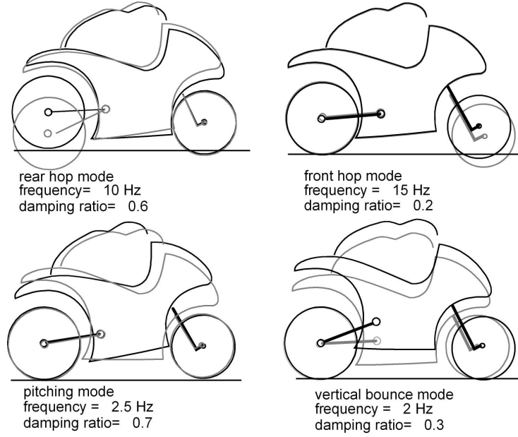
Figure 1.15 In-plane vibration modes.
