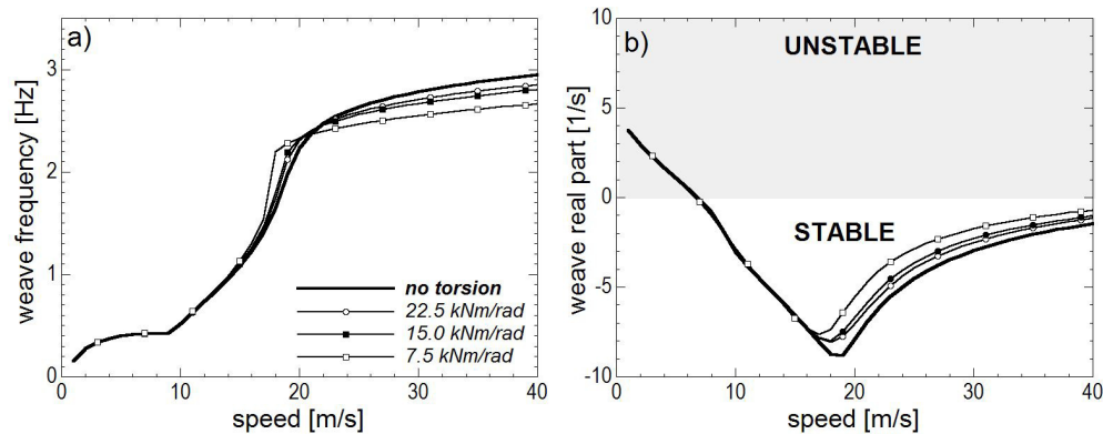
Figure 1.31 Effect of rear torsion on weave.
