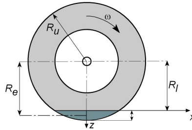
Figure 1.5 Tyre radii.
