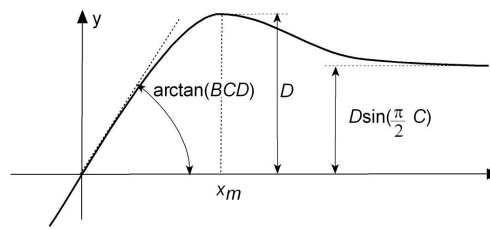
Figure 1.6 Main parameters of the tyre Magic Formula.
